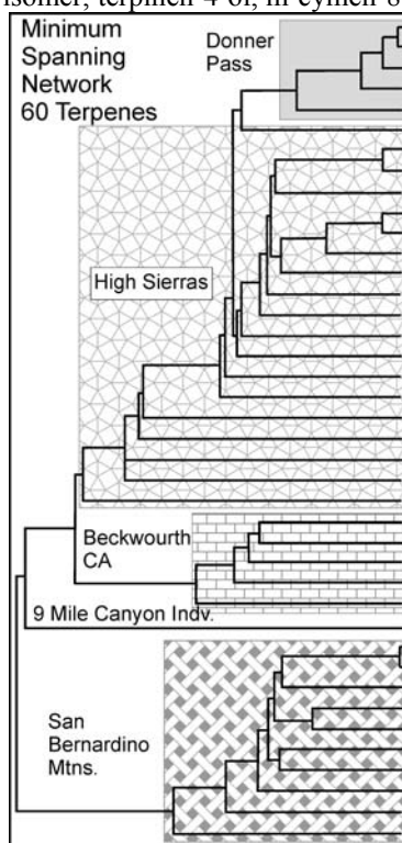
Figure 3. Minimum spanning network based on 60 terpenes.
